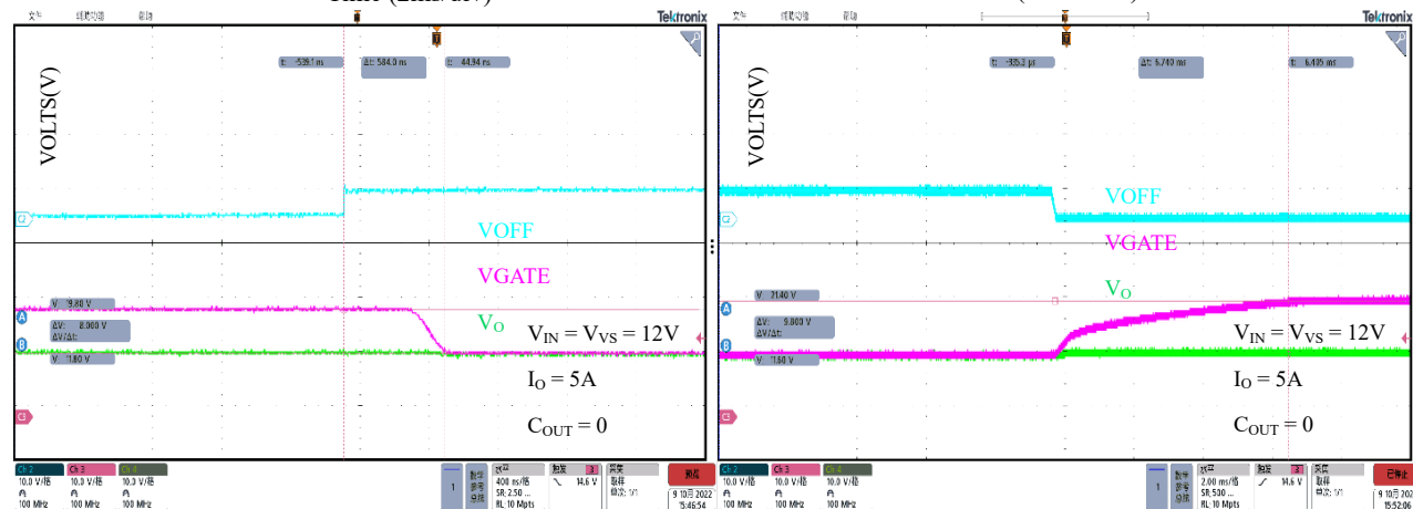
Time (400ns/div)
